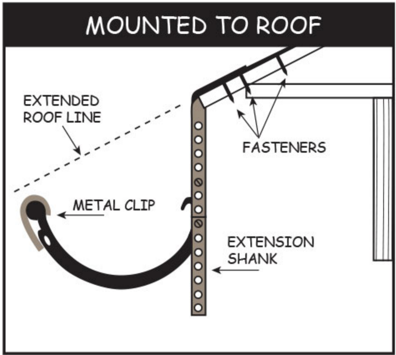
Example of Extension Shank With # 12 Shank
