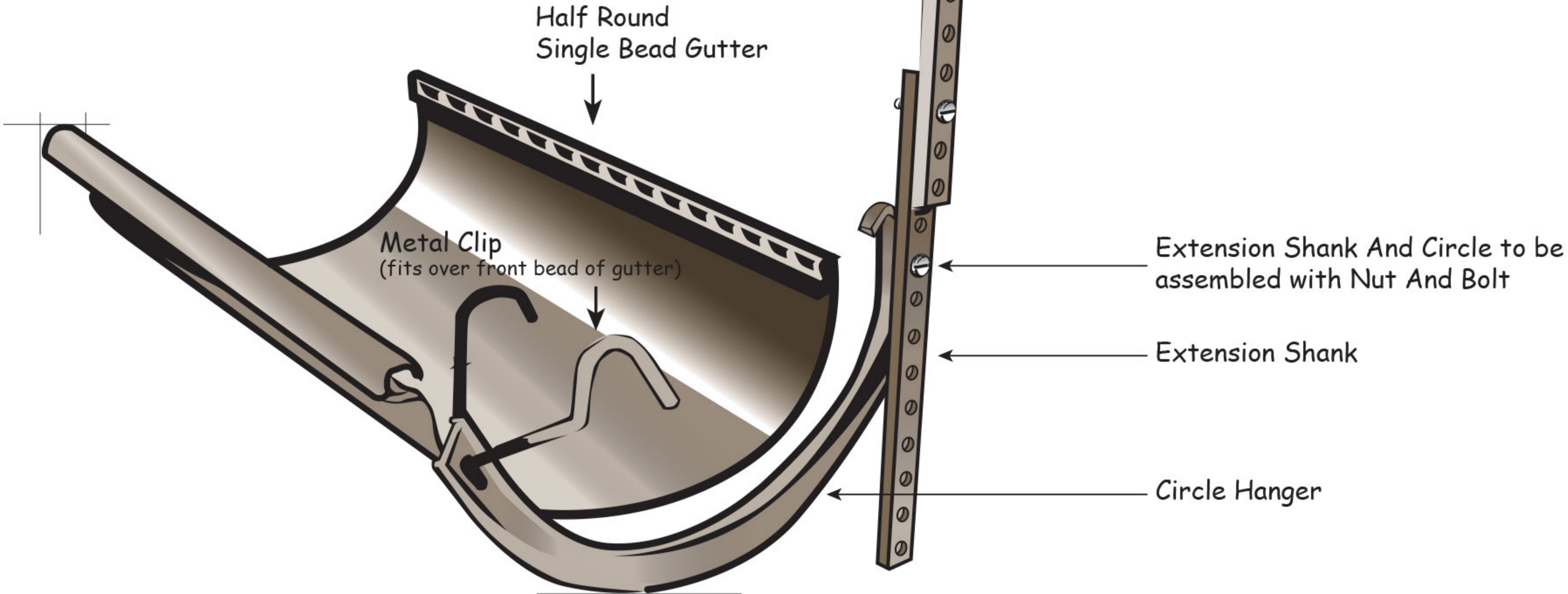
Example of Extension Shank With # 12 Shank
