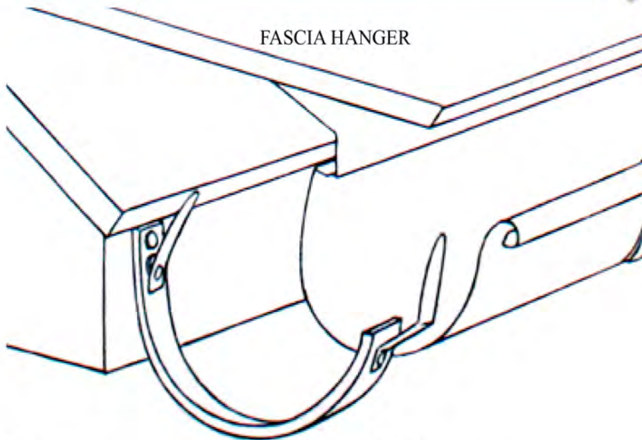
ADJUSTABLE FASCIA HANGER
